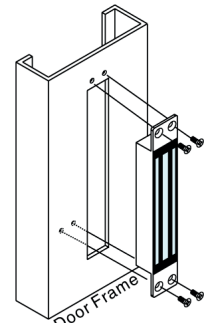
(4) Fix screws
