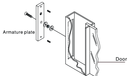
(2) Fix screws
